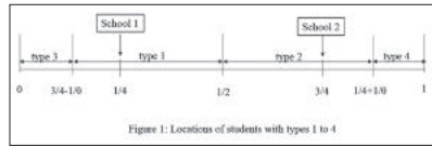
Figure 1: Loci of students with types 1 to 4
